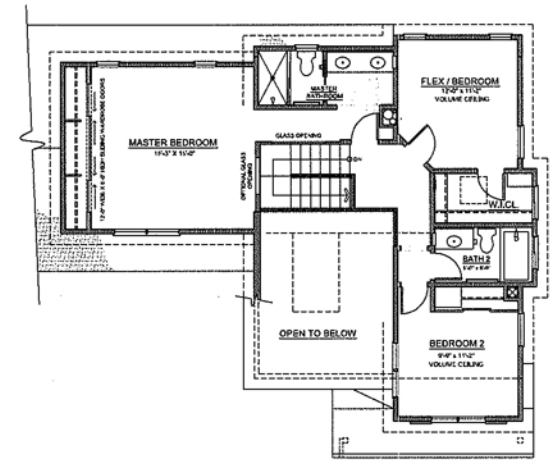
OPTIONAL MASTER BEDROOM OVER GARAGE WITH CLOSET OPTION #1
