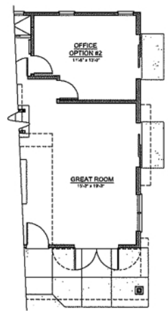
OFFICE OPTION #2
